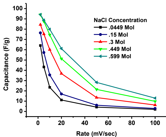
Figure 1. (a) Cyclic voltammety performance of spherical activated carbon based electrodes in different NaCl solutions at 2 \text{ mV s}^{-1} . (b) Rate performance of CDI electrodes in different NaCl concentrated solutions.
